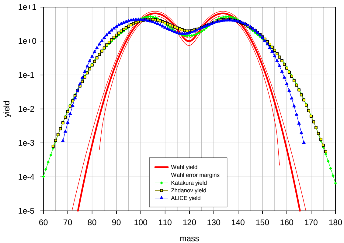
Benchmark B: ^{244}\text{Cm} at 28 MeV, post neutron emission mass distribution
